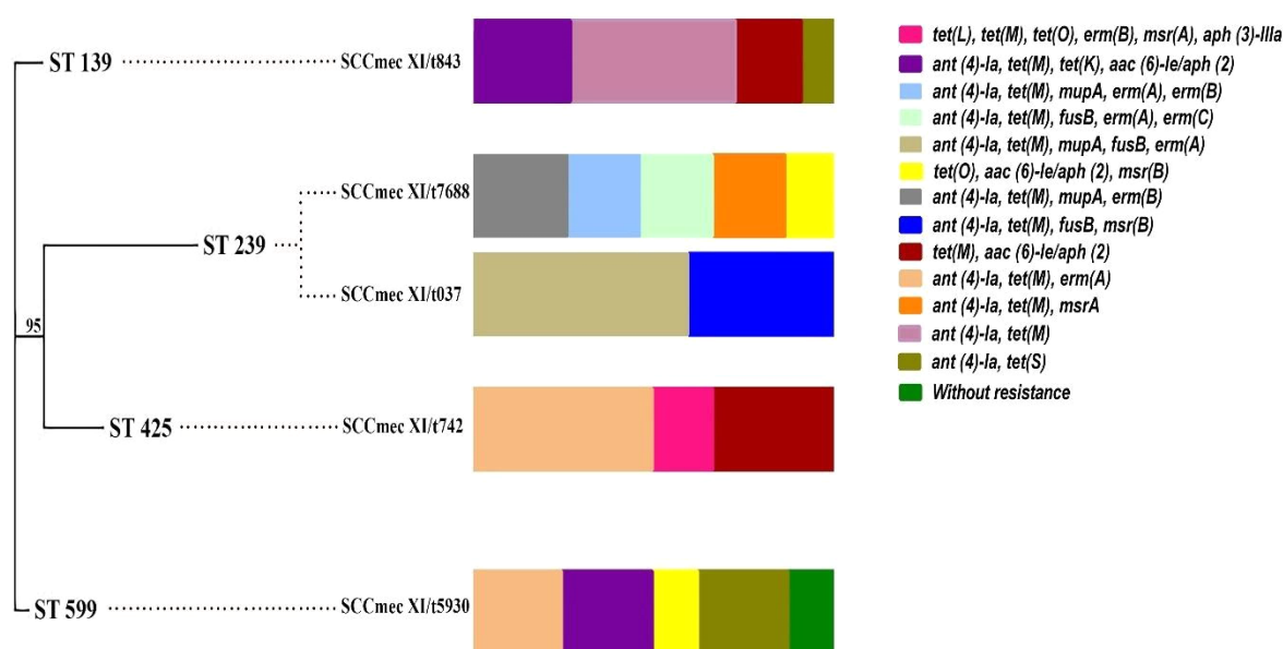
Fig. 5. A phylogenetic tree generated through ML analysis of four STs, using a combination of seven loci ( ArcC , AroE , GlpF , Gmk , Pta , Tpi , and YqiL ). The analysis was conducted with the IQTREE software, applying the TPM2u+F+I model and performing 10,000 ultrafast bootstrap replicates. Bootstrap values greater than 95% are indicated on the tree. ST 239 included two strains that showed different genetic resistance patterns.
