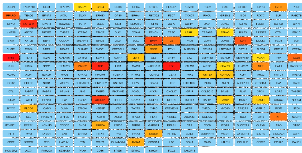
Fig. 5. Protein-protein interaction network of overlapping DEGs between two datasets. Thirty genes with the highest degree are shown in red to yellow color and others are shown in blue.
