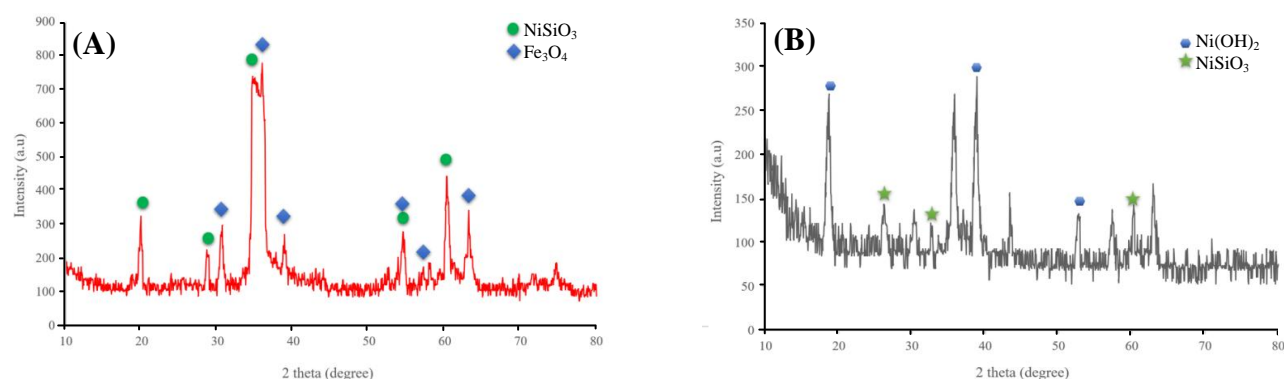
Fig. 3. XRD patterns of nanoparticles. (A) the XRD pattern of \text{Fe}_3\text{O}_4@ \text{NiSiO}_3 and \text{Fe}_3\text{O}_4@ \text{Ni}_x\text{SiO}_y with corresponding picks for \text{NiSiO}_3 and \text{Fe}_3\text{O}_4 and (B) the XRD pattern for \text{Ni}(\text{OH})_2 and \text{NiSiO}_3 , respectively.
