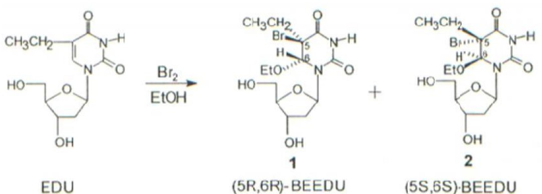
SCHEME 1. Synthesis of the (5R,6R)-1 and (5S,6S)-2 5-bromo-6-ethoxy-5,6-dihydro derivatives of 5-ethyl-2'- deoxyuridine (EDU).
