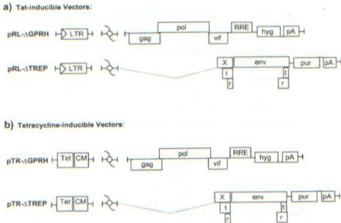
Fig. 1. HIV-2 packaging vectors. This figure shows two sets of HIV-2 'split-genome' packaging vectors. (a) Tat-inducible vectors: pRL- GPRH, a proviral deletion mutant clone with intact 5'LTR, main splice donor site, structural gag-pol genes and accessory vif gene and rev-responsive element (RRE), but it lacks the packaging sequences, and the env gene and 3' LTR which are replaced by the antibiotic selection gene, hygromycin ( hyg ), and a heterologous polyadenylation signal ( pA ). The clone pRL-TREP, also with a deletion of the packaging sequence, has a large deletion of the structural genes, contains intact envelop ( env ), regulatory ( tat and rev ), and antibiotic selection, puromycin ( pur ), genes, and a heterologous polyadenylation site. (b) Tetracycline-inducible vectors: pTR-GPRH and pTR-TREP, are same vectors as in (a) above, except that the 5'LTR gene is replaced by a tetracycline inducible gene fused to a heterologous human cytomegalovirus (CM) promoter. The boxes represent approximations of the size and position of each gene, thus are not drawn to scale.
