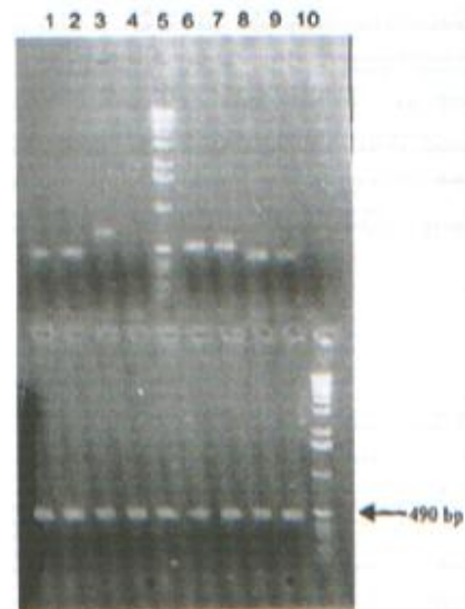
Fig. 2. PCR amplification of ITS2 region in main anopheline malaria vectors from different provinces in Iran. Upper gel: (1, 2), An. pulcherrimus ; (3), An. multicolor ; (4), An. stephensi ; (5), Molecular Marker; (6 & 7), An. fluviatilis ; (8 & 9), An. maculipennis , (10), negative control. Lower gel: An. pulcherrimus from different collection sites in Sistan and Baluchistan province, Iran.
