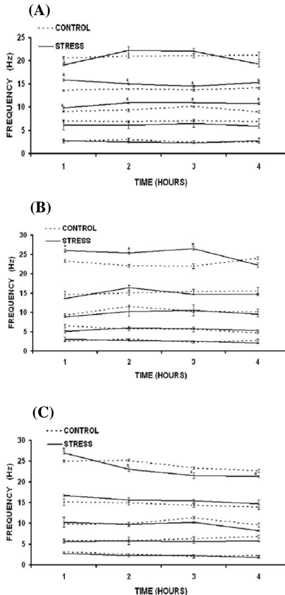
Fig. 1. Data shown in mean ± S.E (n = 5, for both stressed and control groups). Figures show the EEG frequencies of all five bands ( \beta_2 , \beta_1 , \alpha , \theta and \delta ) in (A), SWS; (B), REM sleep and (C), AWA state, following acute heat stress ( *P < 0.05 compared to respective control groups).
