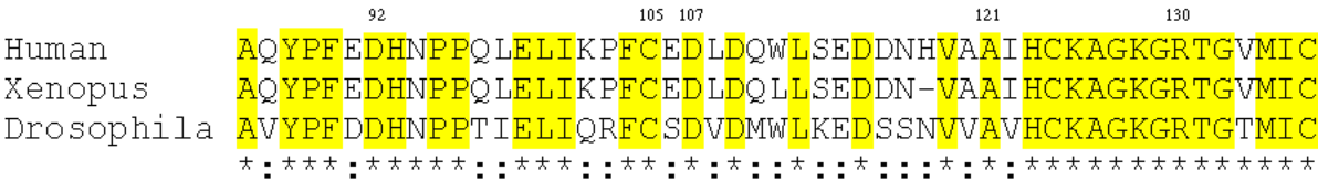
Fig. 4. Multiple alignment of PTEN in human, xenopus and drosophila homologous proteins show the extent of sequences conservation in exons 5 (codon 85-164). Mutations of the six residues (D92, C105, D107, W111, A121 and R130) implicated in sporadic breast cancer patients are conserved among other gene families (shown with codon number).
