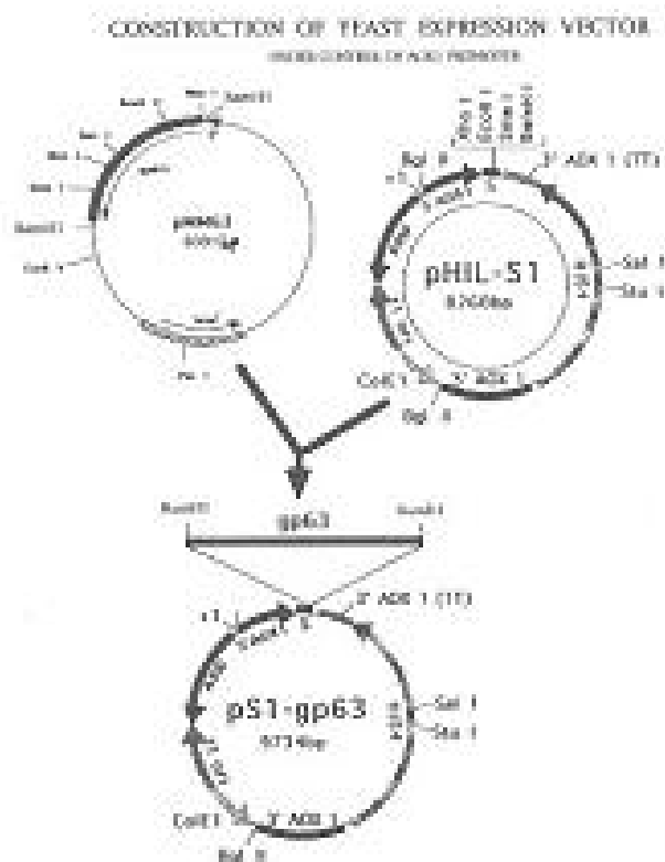
Fig. 1. Schematic diagram of subcloning modified gp63 gene in Bam HI site in MCS of pS1-gp63.
