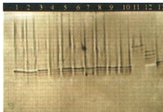
Fig. 3. Electrophoretic patterns obtained for MDH. No. 1, reference strain (RS) of C. luciliae ; No. 2-9, different isolates; No. 10 and 13, RS of L. major ; No. 11, RS of L. infantum ; No. 12, RS of L. tropica .
