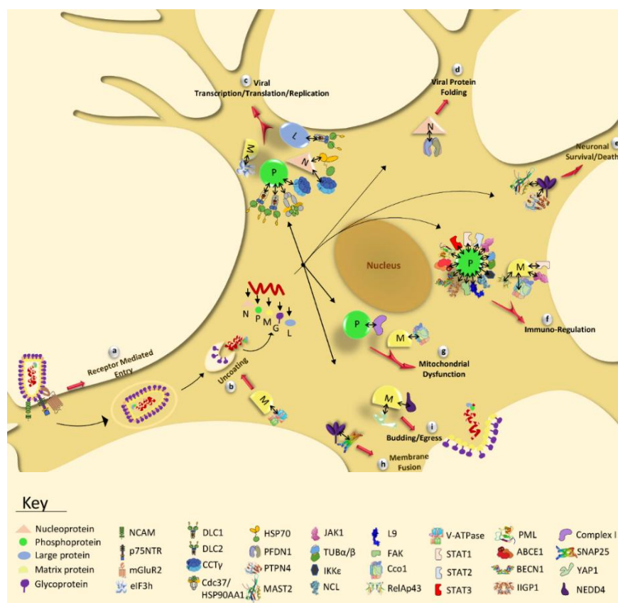
Fig. 7. The lyssavirus-host experimentally defined PPIs and their functional/pathologic outcomes in rabies infection indicated in a neuron. G (glycoprotein), N (nucleoprotein), L (RNA-dependent polymerase or Large protein), P (phosphoprotein), and M (matrix protein) represent five viral proteins which interact with host proteins and facilitate receptor mediated entry of lyssavirus (a), uncoating (b), viral transcription/translation/replication (c), viral protein folding (d), neuronal survival/death (e), immuno-regulation (f), mitochondrial dysfunction (g), membrane fusion (h), and budding (i) during infection. Contribution of the identified PPIs in the mentioned processes has been displayed in the figure and explained in the text. The association of viral-host proteins is shown by right-leftwards arrows in black.
