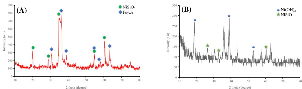
Fig. 3. XRD patterns of nanoparticles. (A) the XRD pattern of \text{Fe}_3\text{O}_4@NiSiO_3 and \text{Fe}_3\text{O}_4@Ni_xSiO_y with corresponding picks for NiSiO_3 and Fe_3O_4 and (B) the XRD pattern of for Ni(OH)_2 and NiSiO_3 , respectively.
