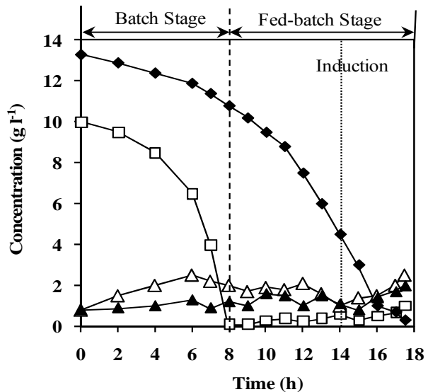
Fig. 5. Effect of feeding strategy on concentration of the main medium components (g l -1 ). Concentration of phosphate (◆), glucose (□), acetate (Δ), and ammonium (▲), in induced recombinant E. coli BL21 (DE3) [pET23a-hgcsf].
