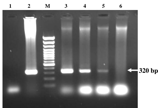
Fig. 2. The inhibitors present in stool inhibited amplification of Blood DNA. Dilution effect in removing inhibitors from amplification reaction of \beta -actin PCR. Lane 1, negative control; Lane 2, positive control (0.5 \mu l blood DNA); Lane M, 100 bp DNA ladder (Fermentas, Lithuania); Lane 3, (0.5 \mu l stool DNA + 0.5 \mu l blood DNA), maximum band intensity, Lane 4, (1 \mu l stool DNA + 0.5 \mu l blood), the bands intensity decreased; Lane 5, (2 \mu l Stool DNA + 0.5 \mu l blood DNA), weak amplification and Lane 6, (3 \mu l stool DNA + 0.5 \mu l blood DNA) no amplification.
