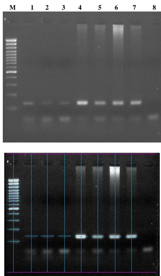
Fig. 1. Comparison in amplification of Exon 9 of TP53 using Stool DNA extracted from one of normal individuals and one of CRC affected Patients. M, 100 bp DNA ladder (Fermentas, Lithuania); Lane 1, normal, Machiels et al. protocol; Lane 2, normal, Ito et al. protocol; Lane 3, normal, our protocol; Lane 4, patient, Machiels et al. protocol; Lane 5, patient, Ito et al. protocol; Lane 6, patient, our protocol; Lane 7, blood sample as positive control; Lane 8, negative control; And at the right hand, band integrity analysis of the samples was shown that is prepared by Kodak Image Analyzer software 1.0.
