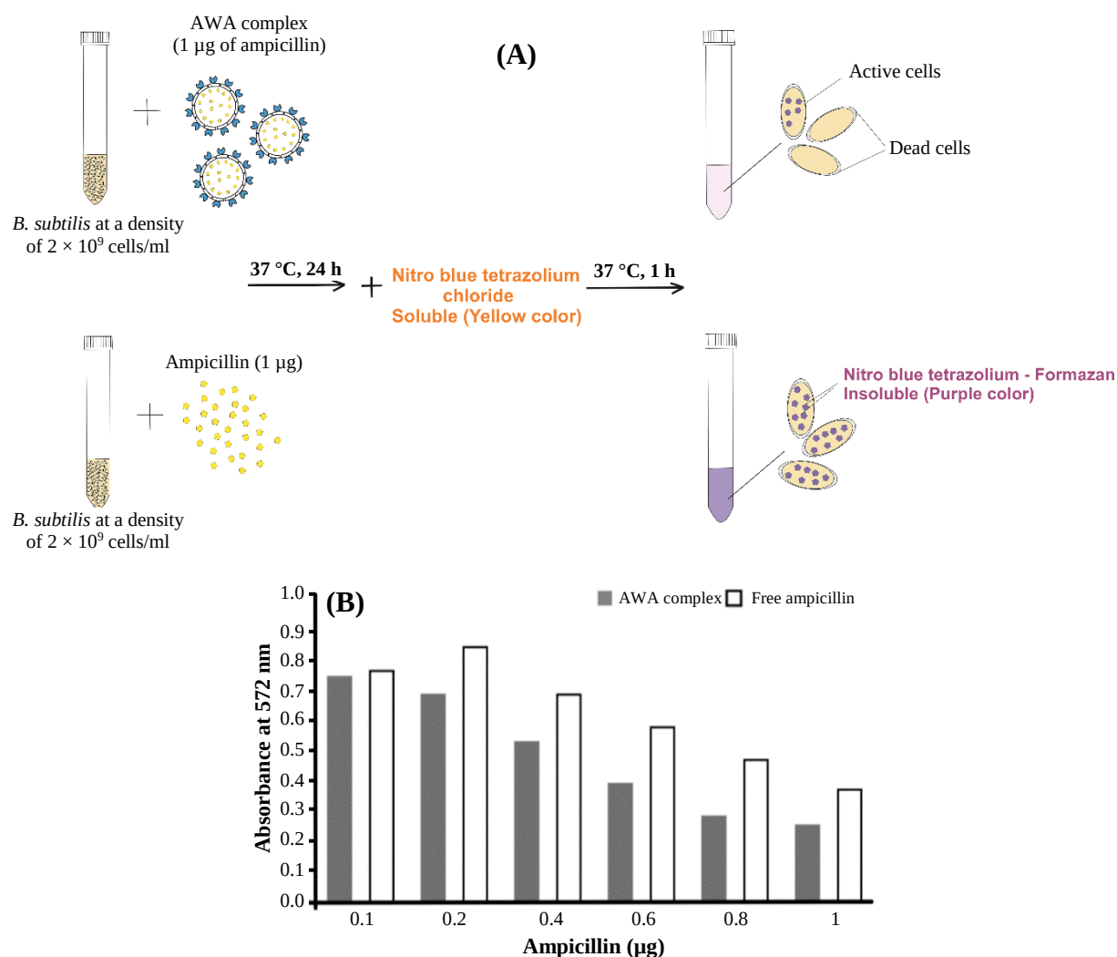
Fig. 3. (A) Quantification of B. subtilis cells via nitroblue tetrazolium analysis; (B) the difference in antibacterial effectiveness between conjugated antibiotic and its free form. Increasing the antibiotic concentration results in a more considerable disparity in their effects.
