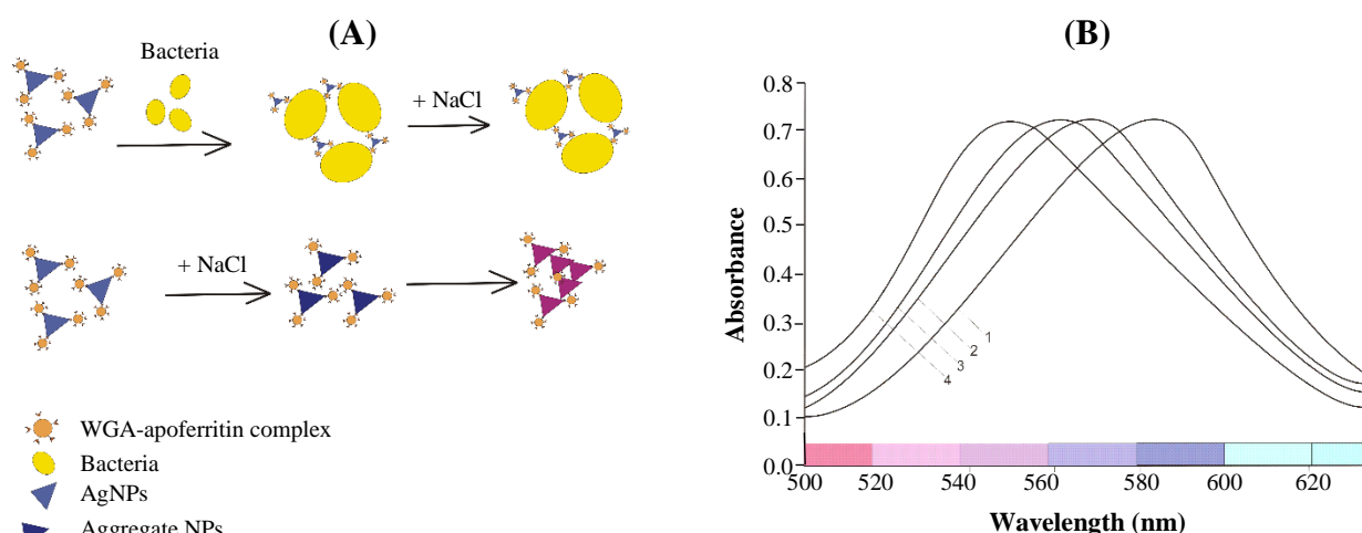
Fig. 2. Detection principle of bacteria binding to AWA-sensitized AgNPs. (A) Schematic representation of the assay using apo ferritin-WGA-sensitized AgNPs; (B) Optical changes observed in apo ferritin-WGA-sensitized AgNPs in the presence of various concentrations of bacteria: 1: 1 \times 10^6 ; 2: 2 \times 10^5 ; 3: 4 \times 10^4 ; 4: no bacteria.
