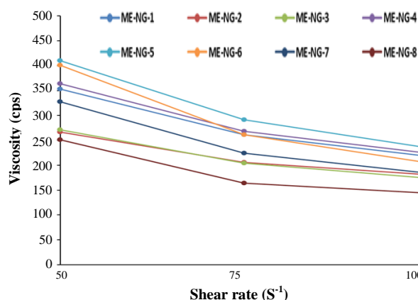
Fig. 5. Rheogram viscosity (cps) versus the shear rate of MEs at 25 °C (mean ± SD of triplicate experiments).
