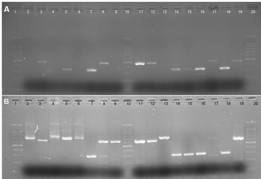
Fig. 2. PCR pattern of G and P type human rotavirus. PCR amplicon of rotavirus typing (A) Representative agarose gel electrophoresis of PCR products of semi-multiplex P typing. Lanes 1, 10, and 20, 100 bp ladder; lane 18, RV4 (P8) representing positive control; lanes 3, 8, 11, 12, 17, and 19, P[4] genotype; lanes 5, 7, 14, 15, and 16, P[8] genotype; lane 2, negative control. Lanes 4, 9, and 13, negative results. (B) Representative agarose gel electrophoresis of PCR products of semi-multiplex G typing. Lanes 1, 10, and 20, 100 bp ladder; lane 2, RV4 (G1) representing positive control; lanes 4, 5, and 6, G1 genotype (749 bp); lanes 3, 8, 9, 11, 12, and 19, G2 genotype (652 bp); lanes 7, 14, 15, and 18, G9 (305 bp); lanes 17, 16, and 13, negative results.
